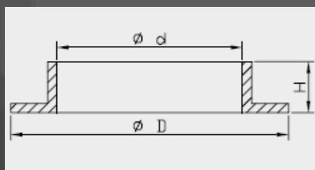
Washer Seal Head Large / Oil Lock dimensions
