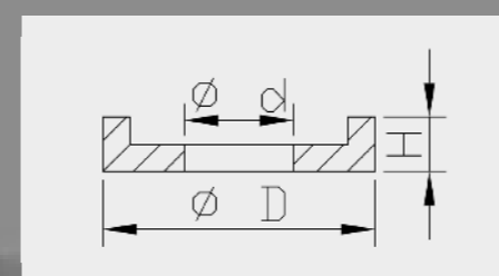
Valve Stopper Compression Base Valve dimensions
